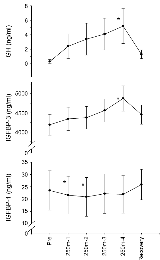
Figure 2. The effect of the sprint interval exercise on circulating growth hormone (GH), insulin-like growth factor binding protein (IGFBP)-3, and IGFBP-1 levels. Exercise was associated with a significant increase of GH and IGFBP-3 and with a significant decrease in IGFBP-1 (* p < 0.05 ). Values returned to baseline levels during recovery.
